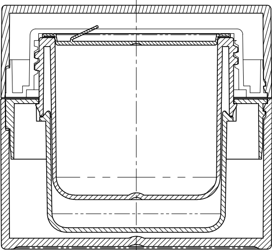
SEC B-B
